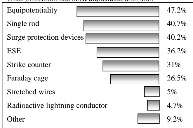
Figure 3: Type of protection
