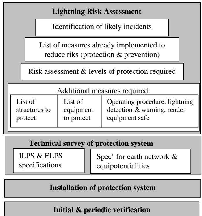
Figure 10: Lightning protection timeline
